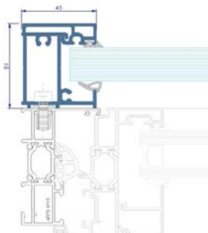
INTEGRATED LATERAL CROSS-SECTION WITH THERMIA HABITAT AR78 SYSTEM
