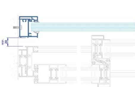
LATERAL CROSS-SECTION WITH SYSTEM THERMIA MAGNA CR46 SLIDING
