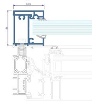
INTEGRATED LATERAL CROSS-SECTION WITH THERMIA LUMIA OC78 SYSTEM
