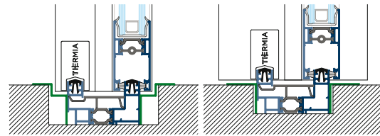
Recessed lower frame.
