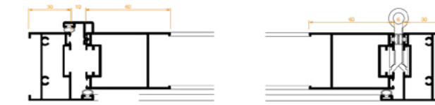
Cross-section single panel
