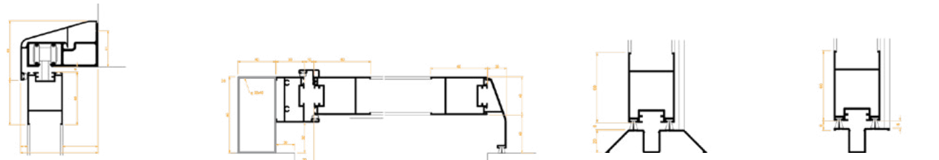
Wall guide with decorative cover Cross-section single panel Overlapping lower guide Embedded lower guide
