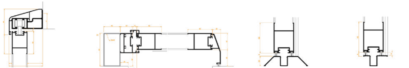
Wall guide with decorative cover Cross-section single panel Overlapping lower guide Embedded lower guide
